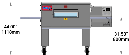
FRONT VIEW - EDGE2440-1
