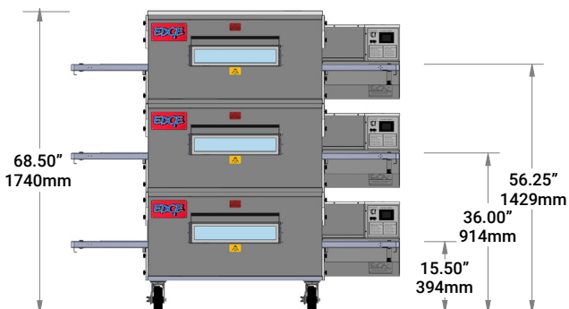
FRONT VIEW - EDGE2440-3
