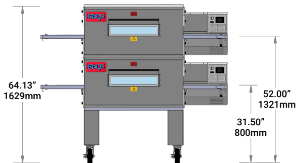
FRONT VIEW - EDGE2440-2
