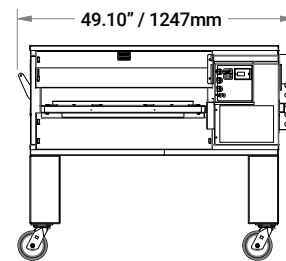
SIDE VIEW - EDGE2440-1
